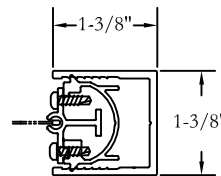
FULLY ASSEMBLED RECESSED SIDE TRACK
