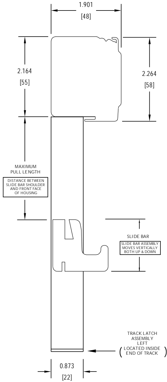
PRESTIGE WINDOW SCREEN ASSEMBLY LEFT SIDE VIEW
