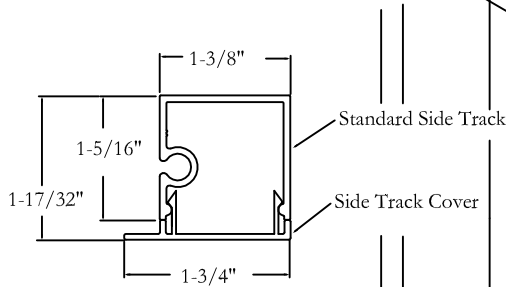
CROSS SECTIONAL VIEW OF THE STANDARD SIDE TRACK (V2A)
