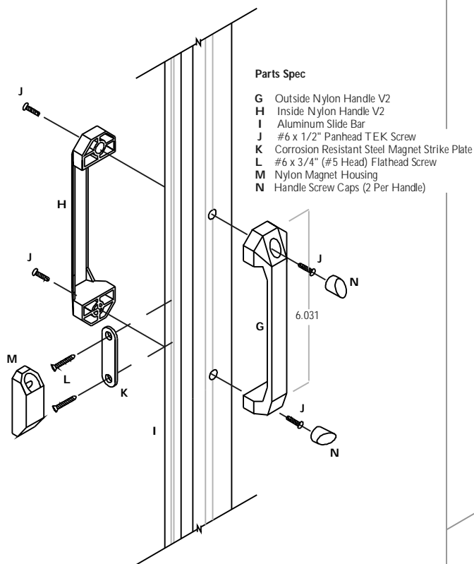
DETAIL OF HANDLE AND STRIKE PLATE POSITION IN RELATION TO THE SLIDE BAR
