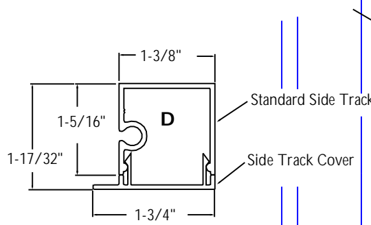
CROSS SECTIONAL VIEW OF THE STANDARD SIDE TRACK (V2A) Scale: 1 : 1
